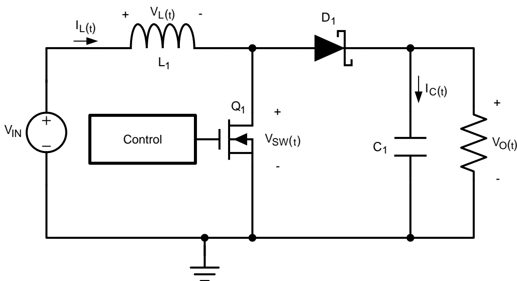
Figure 13. Simplified Schematic
