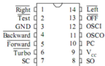
14-Pin DIP/14-Pin SOIC
